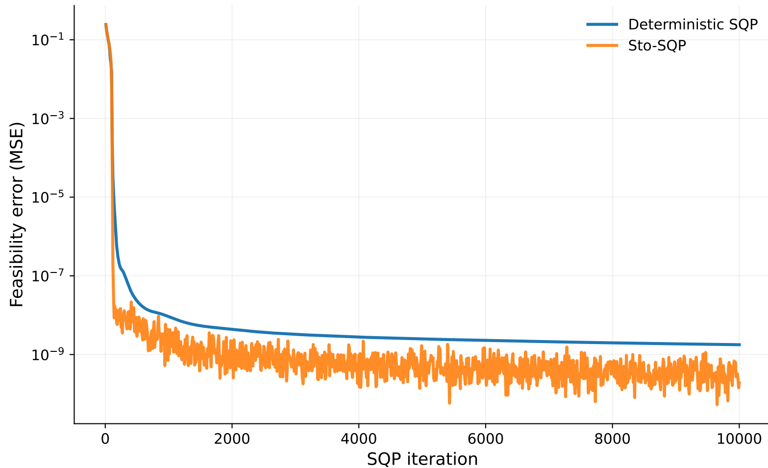
Burgers equation: feasibility error — full trajectory
