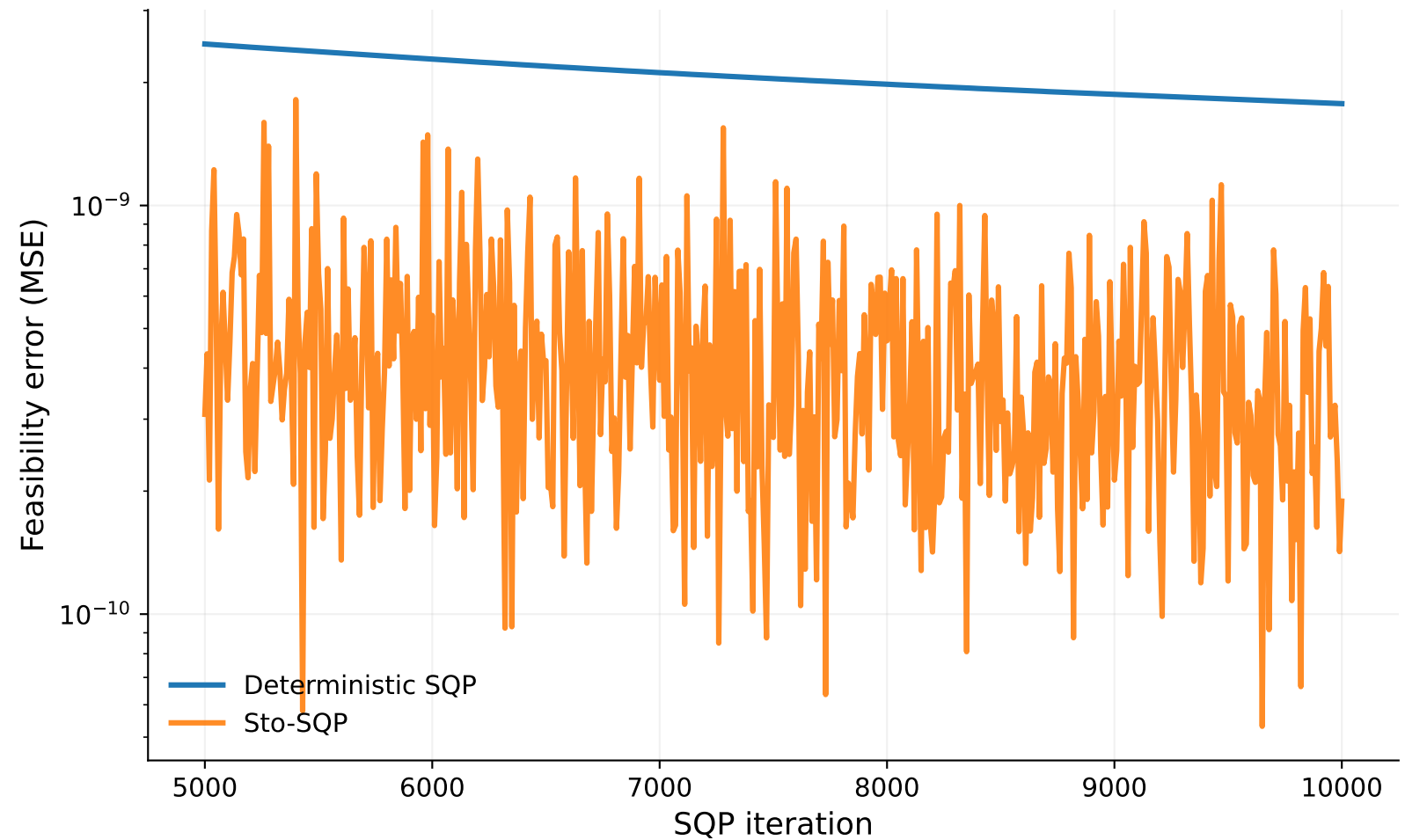
Burgers equation: feasibility error — zoom: iter \geq 5000
